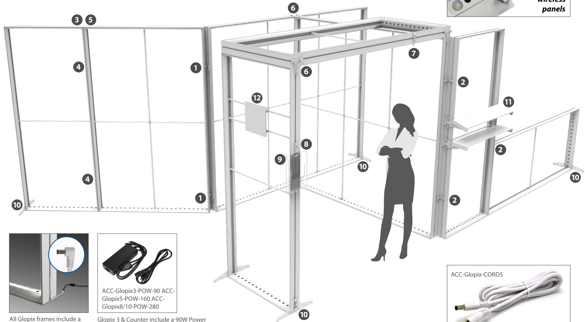
All Glopix frames include a 10" right angle flat DC cable
